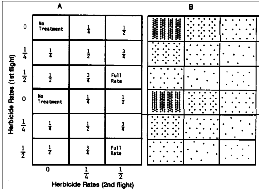
Figure 3. Variable rate pattern (VRP) herbicide treatment showing the variety of cumulative rates for the two perpendicular flights (A) and the simulated vegetation responses (B).
